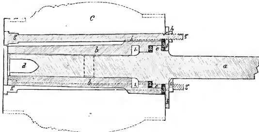
STRATTON'S PATENT MAIL-AXLE.
